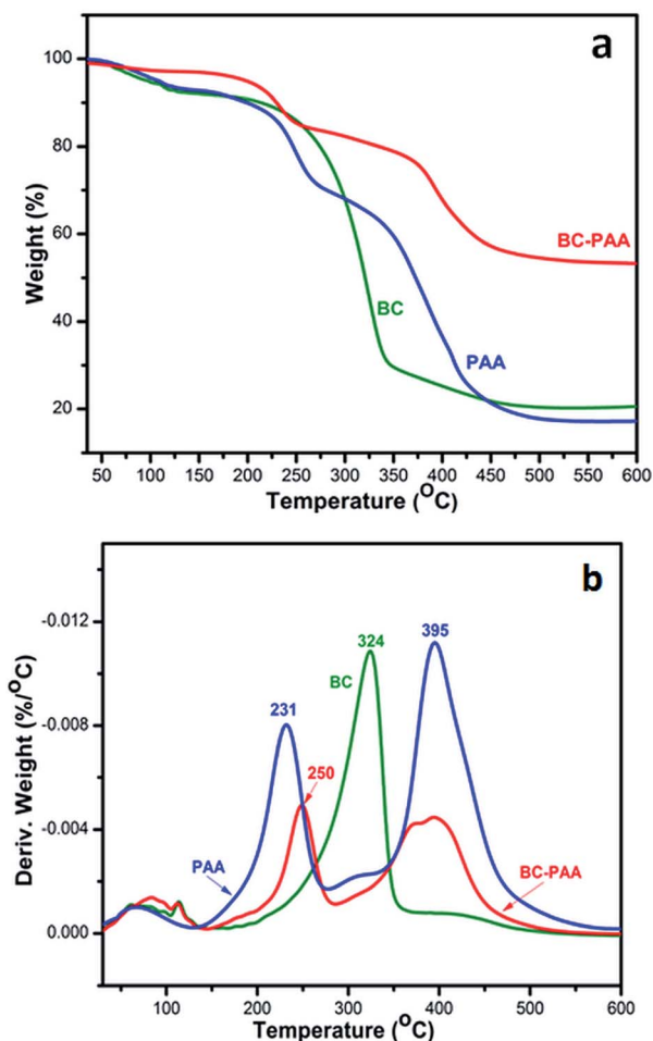
Fig. 2 TGA (a) and DTG (b) curves of BC, PAA and BC-PAA.
