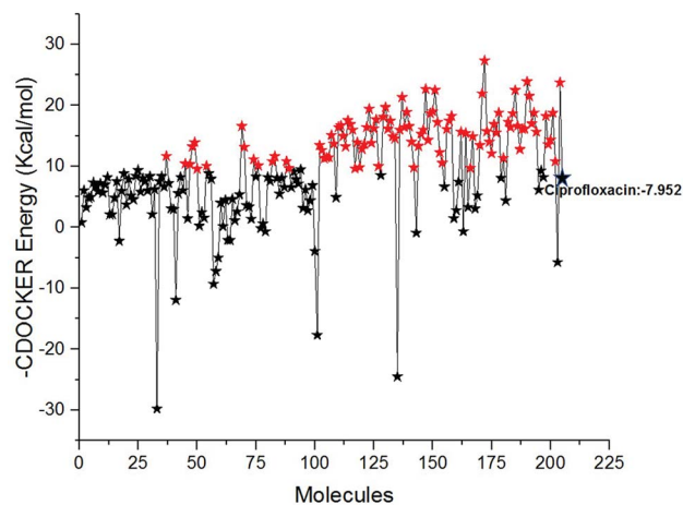
Fig. 6 The–CDOCKER energy score (kcal mol -1 ) of the 204 newly designed FQ analogs. Color code: red stars indicates selected 100 hit compounds having lower–CDOCKER energy ( -9.55 to -29.724 kcal mol -1 ). Black stars indicated the higher–CDOCKER energy compounds ( -9.47 to +29.724 kcal mol -1 ).
