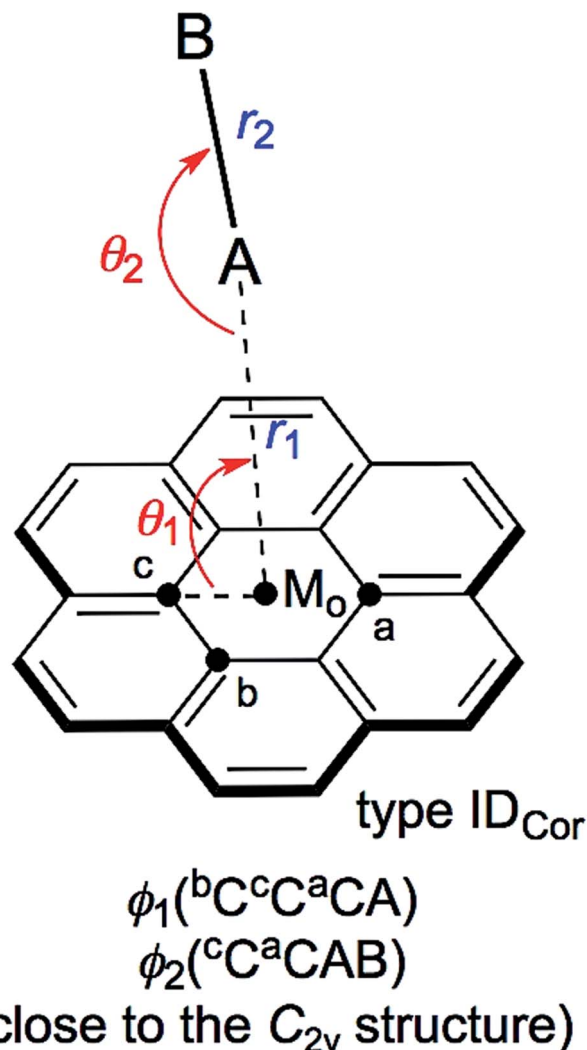
Scheme 2 Structures of \text{X-H}\cdots\pi(\text{C}_{24}\text{H}_{12}) and \text{Y-X}\cdots\pi(\text{C}_{24}\text{H}_{12}) ( \text{A-B} = \text{X-H} or \text{Y-X} ; X, Y = F, Cl, Br and I). The structural parameters are defined, together with the types, where M_o is the centre point of \text{C}_{24}\text{H}_{12} .
