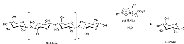
Scheme 1 Cellulose hydrolysis to glucose using Brønsted acidic ionic liquids as both solvent and acidic catalysts.
