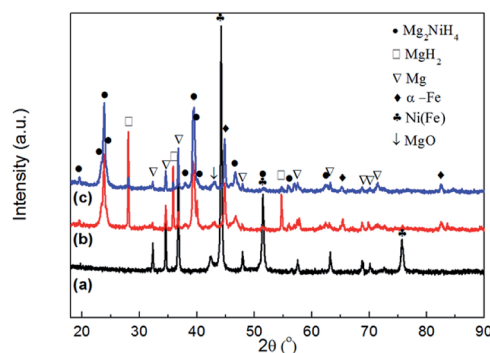
Fig. 4 XRD patterns of as milled Mg–Ni(Fe) powder (a), the Mg–Ni(Fe)–H powder hydrogenated at 623 K under 3.7 MPa H_2 for 48 h (b), the Mg–Ni(Fe)–H powder hydrogenated at 673 K under 3.7 MPa H_2 for 48 h (c).
