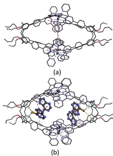
Fig. 4 The optimized structures of \text{Zn}_4\text{L}1_2 (a) and 4(\text{mercaptapurine})@ \text{Zn}_4\text{L}1_2 (b). The interactions are colored in dotted lines: coordination bond in gray, \text{S}-\pi interaction in green, \text{S}-\text{H}-\pi interaction in yellow and \pi-\pi interaction in pink. All hydrogens are omitted for clarity.
