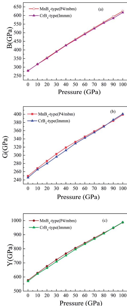
Fig. 5 Calculated elastic modulus of MoB 4 as a function of pressure. (a) Bulk modulus vs. pressure, (b) shear modulus vs. pressure, and (c) Young's modulus vs. pressure, respectively.
