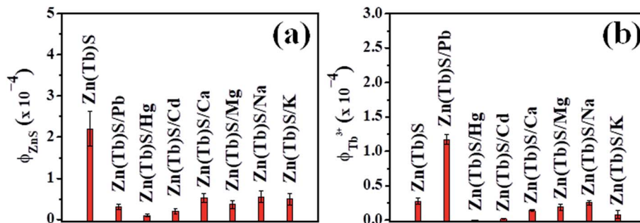
Fig. 11 The trend in the broad and sharp emission of the ZnS nanoparticles (panel a) and Tb^{3+} (panel b), respectively, are shown for cases where the Zn(Tb)S nanoparticles were post-synthetically treated with M^{n+} , with [Zn(Tb)S] : [M^{n+}] = 1 : 10^{-2} . The values reported are average and standard deviation from two independent measurements.
