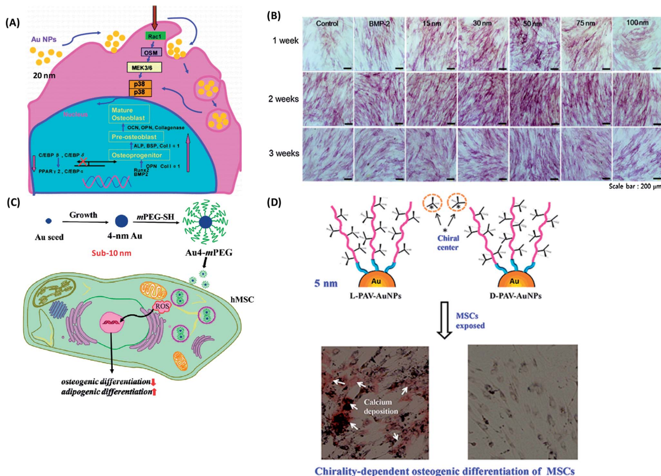
Fig. 5 (A) Molecular mechanism of the modulation of osteogenic and adipogenic differentiation of MSCs by AuNPs through p38 MAPK signaling pathway. Reproduced with permission. 144 Copyright 2010, American Chemical Society. (B) ALP staining and activity level during the process of differentiation from ADSCs toward osteoblasts for 3 weeks: ALP stained cells, which were treated with osteogenic medium alone (control), BMP-2, and each size of GNPs for 3 weeks as observed by an optical microscope. Reproduced with permission. 146 Copyright 2014, Elsevier. (C) Schematic illustrations of the fabrication process of Au4-mPEG NPs, and the possible molecular mechanism of the inhibitive effect of Au4-mPEG NPs on osteogenic differentiation and their promotive effect on adipogenic differentiation. Reproduced with permission. 148 Copyright 2017, Royal Society Chemistry. (D) Schematic diagrams of the effects of the surface chirality at the nanoscale on osteogenic differentiation of MSCs. Reproduced with permission. 150 Copyright 2016, Springer.
