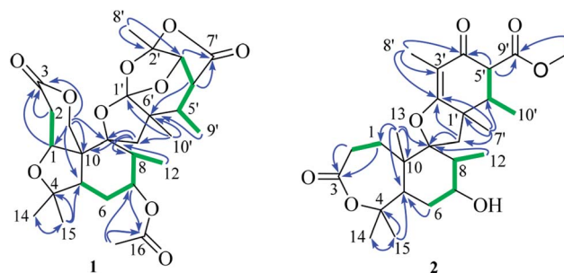
Fig. 2 Key HMBC (blue arrows) and ^1\text{H} - ^1\text{H} COSY (green bold lines) correlations of 1 and 2 .
