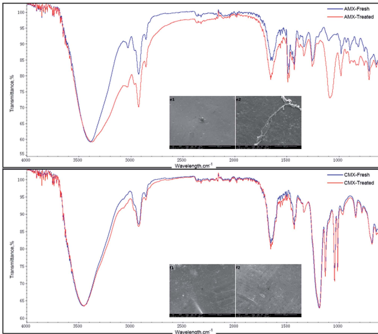
Fig. 11 SEM images and ATR-FTIR spectra of the AMX and CMX membranes before and after the treatment of a nucleotide salt mixture: (e1) fresh and (e2) treated AMX; (f1) fresh and (f2) treated CMX.
