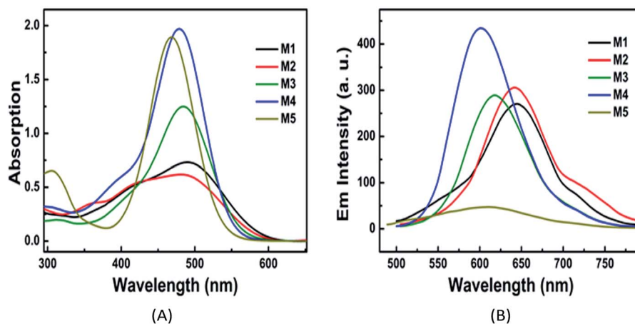
Fig. 2 Absorption (A) and fluorescence (B) spectra of PSs M1–M5 in PBS ( 5.0 \times 10^{-5} \text{ mol L}^{-1} ).
