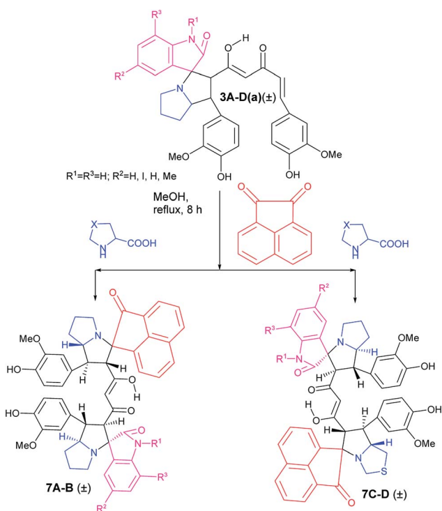
Scheme 4 Synthesis of mixed bis-pyrrolizidino/-thiopyrrolizidino dispiro-oxindolo-acenaphthyleno curcuminoids.
