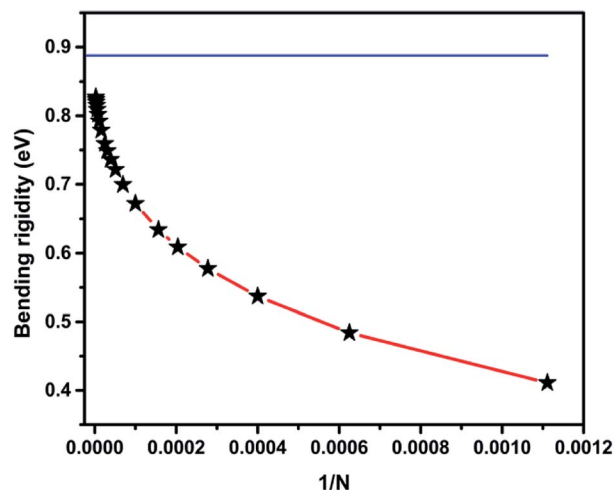
Fig. 3 The variation in bending modulus is inverse to the system size. The blue line represents the bending rigidity value extrapolated to an infinite system size using an equation derived from the Foppl–von Karman theory.
