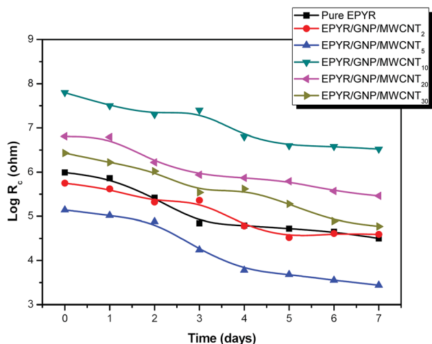
Fig. 9 Change of R_c in accordance with the immersion time for pure EPYR and its corresponding EPYR/GNP/MWCNT 2-30 composite materials.
