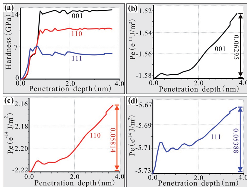
Fig. 3 (a) Nano-hardness of the three different models. (b) Penetration depth–energy curve of the (001) model. (c) Penetration depth–energy curve of the (110) model. (d) Penetration depth–energy curve of the (111) model.
