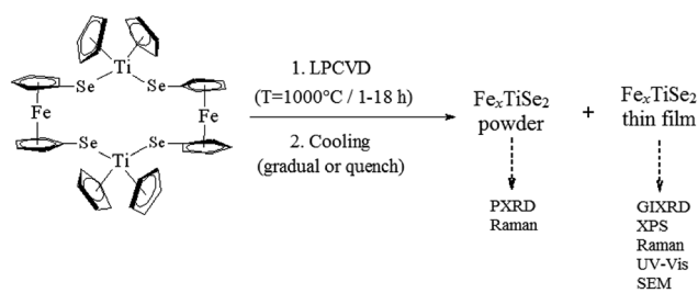
Scheme 1 Scheme of the LPCVD of precursor ( 1 ) and analysis techniques for products (powders and films).
