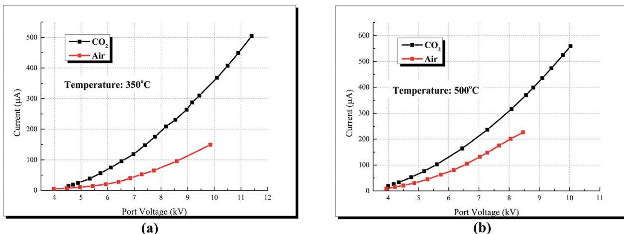
Fig. 7 Effect of gas media on corona discharge current at different temperature. (a) 350\text{ }^\circ\text{C} and (b) 500\text{ }^\circ\text{C} .
