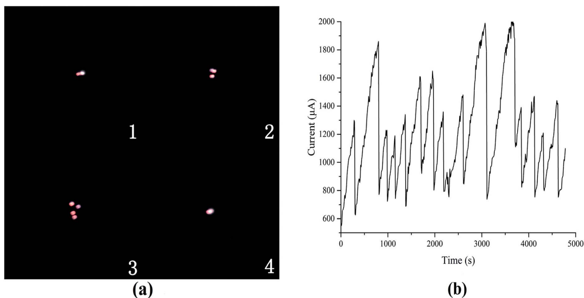
Fig. 13 (a) Discharge photographs and (b) its current curve at 20 ^\circ\text{C} and on the output voltage of 5.5 kV.
