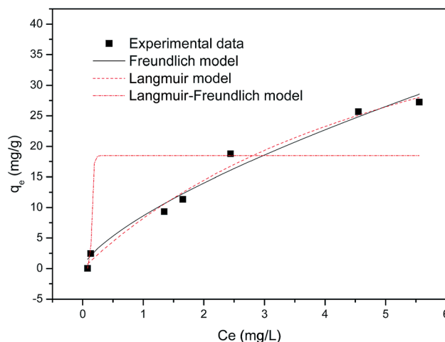
Fig. 4 Adsorption isotherm curves of DMP on biochar.
