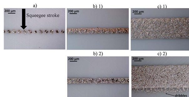
Fig. 5 Photographs of screen printed lines: (a) 50 \mu\text{m} theoretical width line, (b) 100 \mu\text{m} theoretical width line: (1) without defect, (2) with a lack of ink, (c) 500 \mu\text{m} theoretical width line: (1) without defect and (c) (2) with dribbles at the lower edge.
