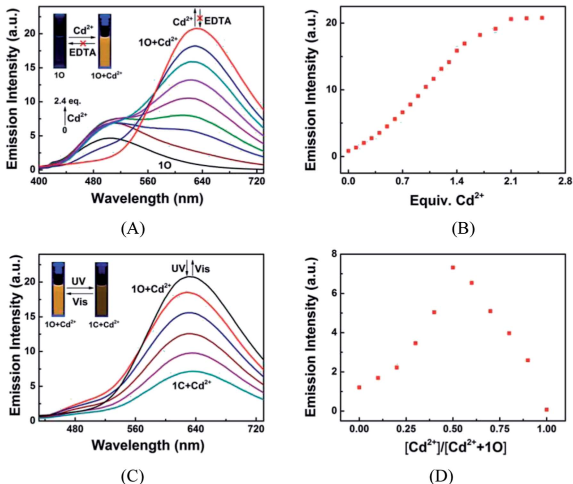
Fig. 5 Fluorescence responses of 1O ( 2.0 \times 10^{-5} mol L -1 ) to Cd 2+ /EDTA in acetonitrile, excited at 392 nm. (A) Fluorescent emission spectra of 1O titrated with different amounts of Cd 2+ ; (B) fluorescence intensities of 1O at 633 nm as titrated with different equiv. of Cd 2+ ; (C) fluorescent emission spectra of 1O + Cd 2+ under alternating photoirradiation with UV and visible light; (D) Job's plot showing the 1 : 1 complex of 1O with Cd 2+ .
