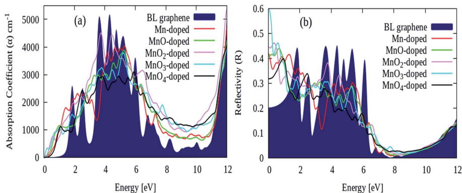
Fig. 7 (a) Absorption coefficient ' \alpha ' and (b) reflectivity ' R ' parameters of pure and different Gr/MnO x /Gr cluster-sandwiched bilayer graphene systems.
