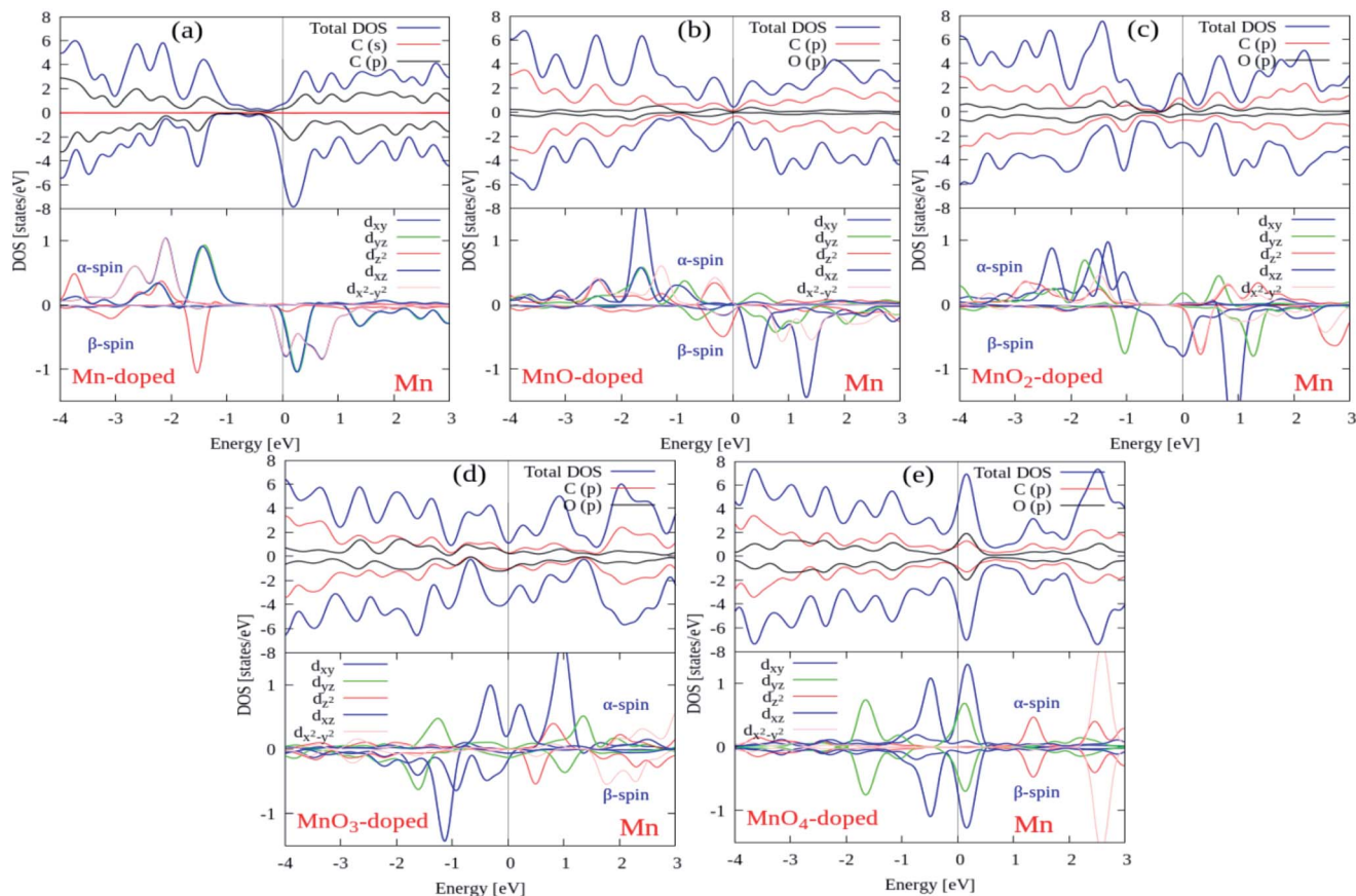
Fig. 5 Total and projected DOS plots for \text{Gr}/\text{MnO}_x/\text{Gr} cluster-sandwiched bilayer graphene systems. The solid grey line appearing at 0 eV energy level depicts the Fermi energy level.
