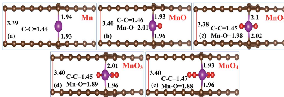
Fig. 1 Side view of the atomic structures of \text{MnO}_x cluster-sandwiched bilayer graphene systems (where, x = 0-4 ). The small black and red balls represent the C and O atoms respectively, and the big ball represents the Mn atom.
