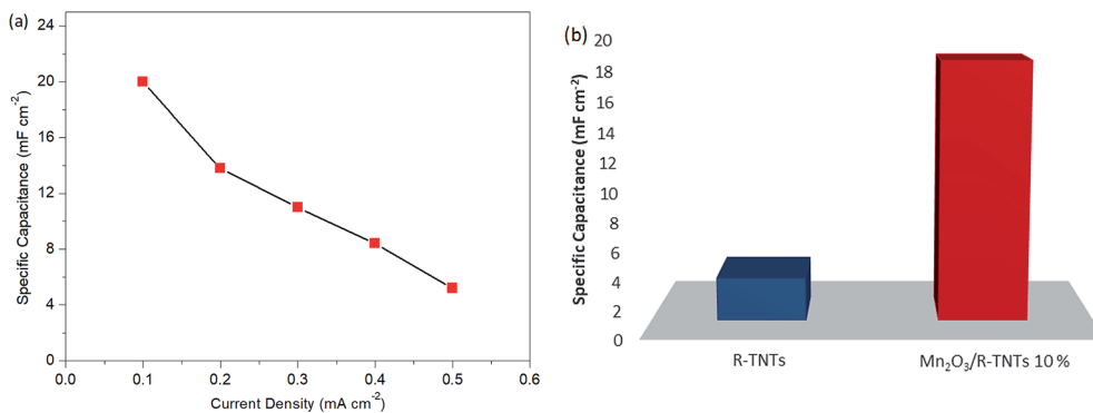
Fig. 8 Specific capacitance of (a) Mn 2 O 3 /R-TNTs deposited at 10% duty cycle at various current densities and (b) R-TNTs and Mn 2 O 3 /R-TNTs synthesized at 10% duty cycle.
