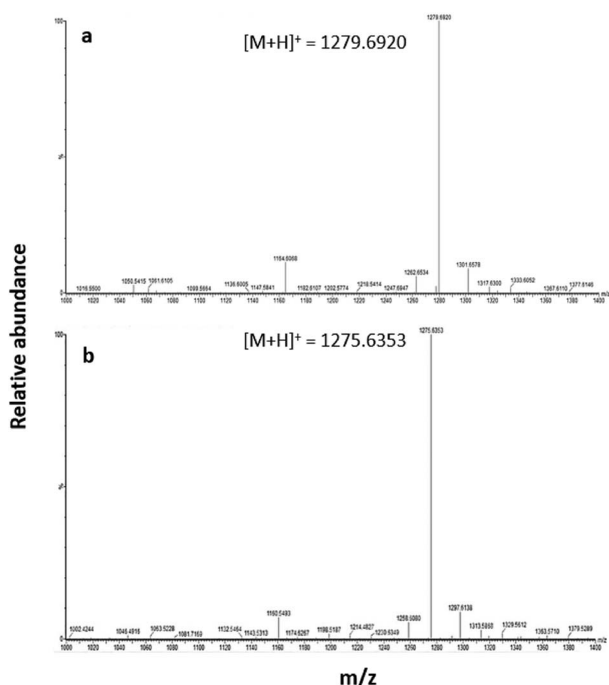
Fig. 2 HR-ESI(+) mass spectra of pure (a) linear It5d with the molecular ion peak at 1279.6920, and (b) folded It5d at 1275.6353. Calculated monoisotopic mass of target linear and folded peptide is 1278.5229 and 1274.4916 Da, respectively.
