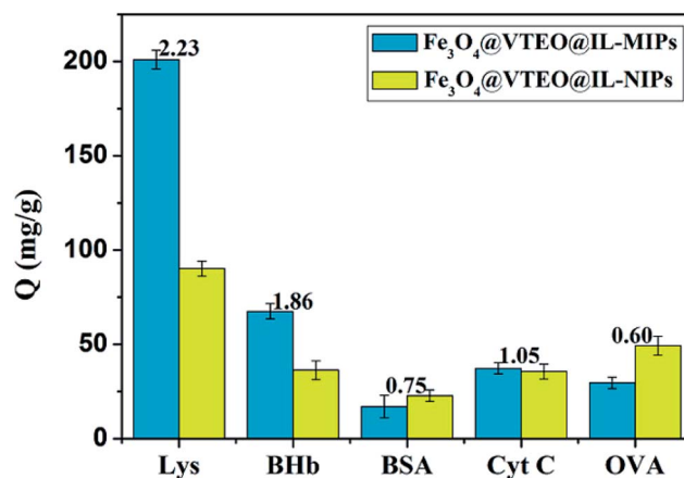
Fig. 5 Adsorption capacities of different proteins on \text{Fe}_3\text{O}_4@V\text{TEO}@IL\text{-MIPs} and \text{Fe}_3\text{O}_4@V\text{TEO}@IL\text{-NIPs} . Adsorption conditions: V = 1 \text{ mL} , m_{\text{MIPs}} = m_{\text{NIPs}} = 5 \text{ mg} , C_0 = 1.4 \text{ mg mL}^{-1} , T = 25 \text{ }^\circ\text{C} , t = 2.5 \text{ h} .
