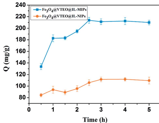
Fig. 4 The adsorption kinetics of Lys on \text{Fe}_3\text{O}_4@V\text{TEO}@IL\text{-MIPs} and \text{Fe}_3\text{O}_4@V\text{TEO}@IL\text{-NIPs} . Adsorption conditions: V = 1 \text{ mL} , m_{\text{MIPs}} = m_{\text{NIPs}} = 5 \text{ mg} , C_{\text{Lys}} = 1.4 \text{ mg mL}^{-1} , T = 25 \text{ }^\circ\text{C} .
