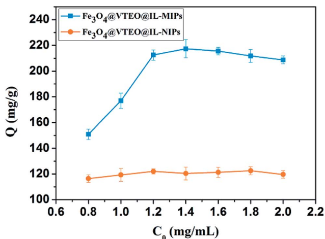
Fig. 3 The adsorption isotherm of Lys on \text{Fe}_3\text{O}_4@V\text{TEO}@IL\text{-MIPs} and \text{Fe}_3\text{O}_4@V\text{TEO}@IL\text{-NIPs} . Adsorption conditions: V = 1 \text{ mL} , m_{\text{MIPs}} = m_{\text{NIPs}} = 5 \text{ mg} , C_{\text{Lys}} = 0.8\text{--}2.0 \text{ mg mL}^{-1} , T = 25 \text{ }^\circ\text{C} , t = 12 \text{ h} .
