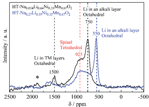
Fig. 3 {}^6\text{Li} -MAS-NMR spectra of \text{HT-Na}_{0.034}\text{Li}_{0.64}\text{Ni}_{0.33}\text{Mn}_{0.67}\text{O}_2 (before chemical lithiation) measured at room temperature. "*" indicates a spinning sideband.
