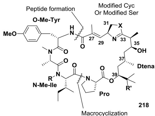
218 a: X=S, R=R'=Me, Apratoxin A 218 b: X=S, R=H, R'=Me, Apratoxin B 218 c: X=S, R=Me, R'=H, Apratoxin C 218 d: X=O, R=R'=Me, Oxazoline analogue of Apratoxin A
