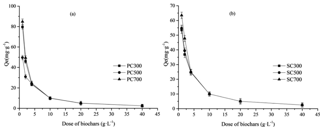
Fig. 4 Effects of biochar mass on the adsorption of Cd(II) by different spent Pleurotus ostreatus substrate biochars (a) and spent shiitake substrate biochars (b). Note: spent Pleurotus ostreatus substrate biochar (PC), spent shiitake substrate biochar (SC).
