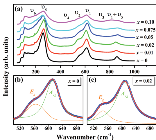
Fig. 3 (a) Room temperature Raman spectra of (1-x)\text{K}_{0.5}\text{Na}_{0.5}\text{NbO}_3-(x)\text{BiZn}_{0.5}\text{Ti}_{0.5}\text{O}_3 ceramics with 0 \leq x \leq 0.10 . Fitted Raman spectrum using the sum of two Lorentzian peaks between 500\text{--}700\text{ cm}^{-1} for (b) x = 0 and (c) x = 0.02 .
