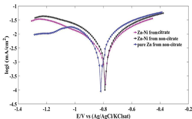
Fig. 7 Polarization curve for the pure Zn and Zn–Ni alloy coatings deposited from citrate and non-citrate baths.
