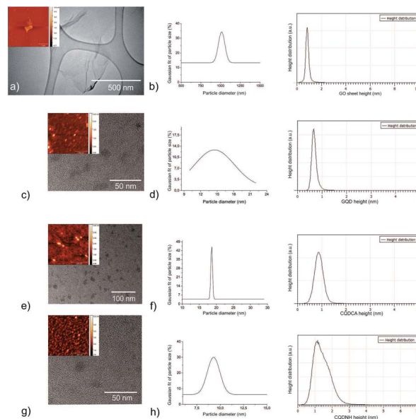
Fig. 1 TEM micrographs, top view AFM images (insets), Gaussian fit of particle size and height distributions of the: (a and b) GO; (c and d) QGDs; (e and f) CQDCA and (g and h) CQDNH samples. The particle size and height of all dots were calculated for set of 100 dots whereas for the GO sample set had 50 GO sheets.
