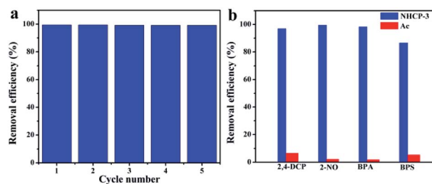
Fig. 6 (a) Reusability of the NHCP-3 for BPA in 30 minutes. (b) Removal efficiency of 2,4-DCP ( 0.1 \text{ mM} ), 2-NO ( 0.1 \text{ mM} ), BPA ( 0.1 \text{ mM} ) and BPS ( 0.1 \text{ mM} ) obtained by rapidly flowing the pollutants solution through NHCP-3 (blue) and Ac (red), respectively. The amount of the adsorbent used in this study is 1 \text{ mg mL}^{-1} .
