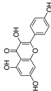
Kaempferol (FLAVONOID)
