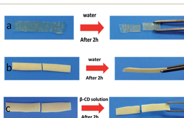
Fig. 10 Self-healing tests using different materials: (a) samples without CD- \text{Al}_2\text{O}_3 NPs; (b) samples without PVP; (c) self-healing test of PVP/p(HEMA-co-BA) after smearing cyclodextrin solution at cutting surface.
