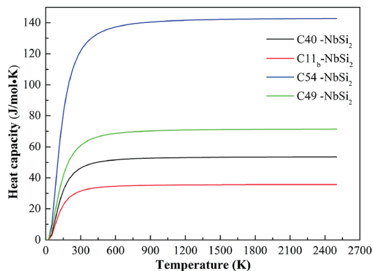
Fig. 5 Calculated the heat capacity ( C_V ) of various \text{NbSi}_2 phases.
