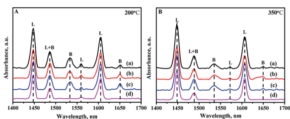
Fig. 9 FTIR spectra of pyridine adsorbed on different catalysts after degassing at (A) 200 °C and (B) 350 °C: (a) NiMo/Zr-in-F, (b) NiMo/Zr-im-F, (c) NiMo/Zr-gra-F, (d) NiMo/Zr-im-F.
