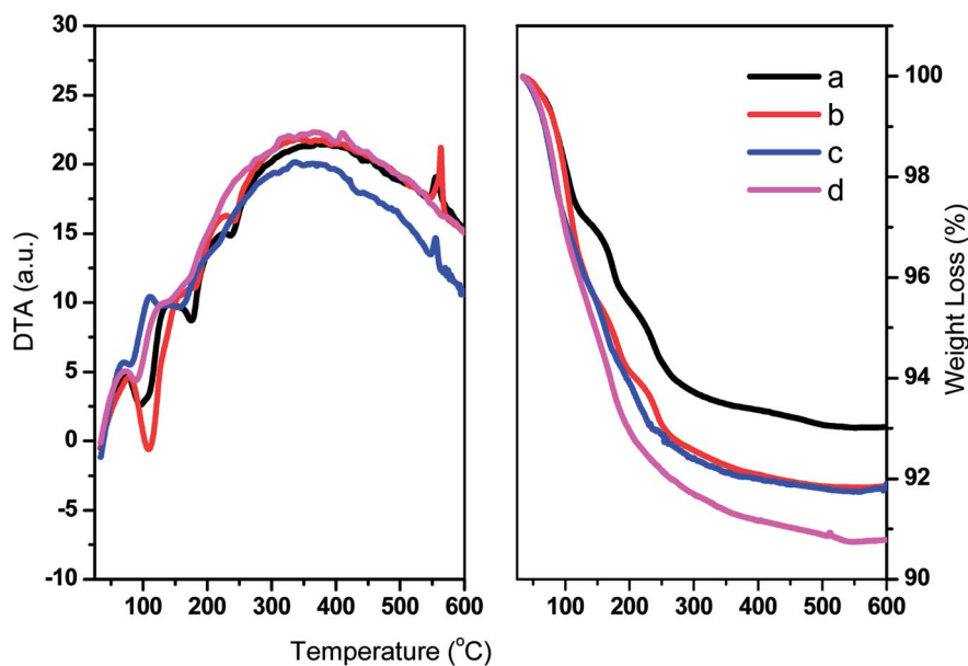
Fig. 5 DTA (left panel) and TGA (right panel) of (a) TPA/ \gamma -Al 2 O 3 , (b) Zn 0.5 TPA/ \gamma -Al 2 O 3 , (c) Zn 1 TPA/ \gamma -Al 2 O 3 , and (d) Zn 1.5 TPA/ \gamma -Al 2 O 3 .
