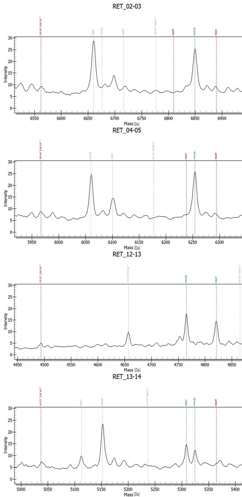
Fig. 4 Array-based MALDI-TOFMS results of RET fusions in the mass spectra of RET 02-03, extended primers were supposed to be detected in 6890 dalton and 6238 in RET04-05, but no cDNA or very few cDNAs were detected in RET 02-03 and RET 04-05, in the mass spectra of RET12-13, extended primers were supposed to be detected in 4821 dalton and 5309 in RET 13-14, and large amounts of cDNAs were detected in RET 12-13 and RET 13-14. By calculating Z score, RET fusion was determined.
