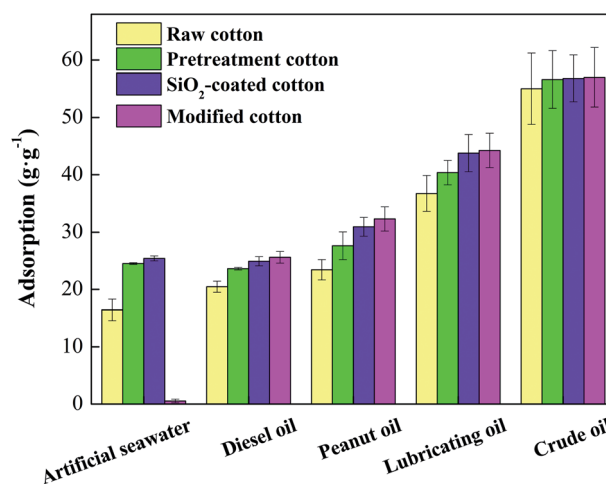
Fig. 5 Adsorption capacity of cotton fiber at different stages.
