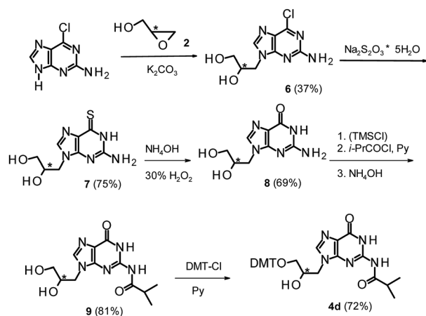
Scheme 2 Synthesis of DMT-G G iBu ( 4d ).
