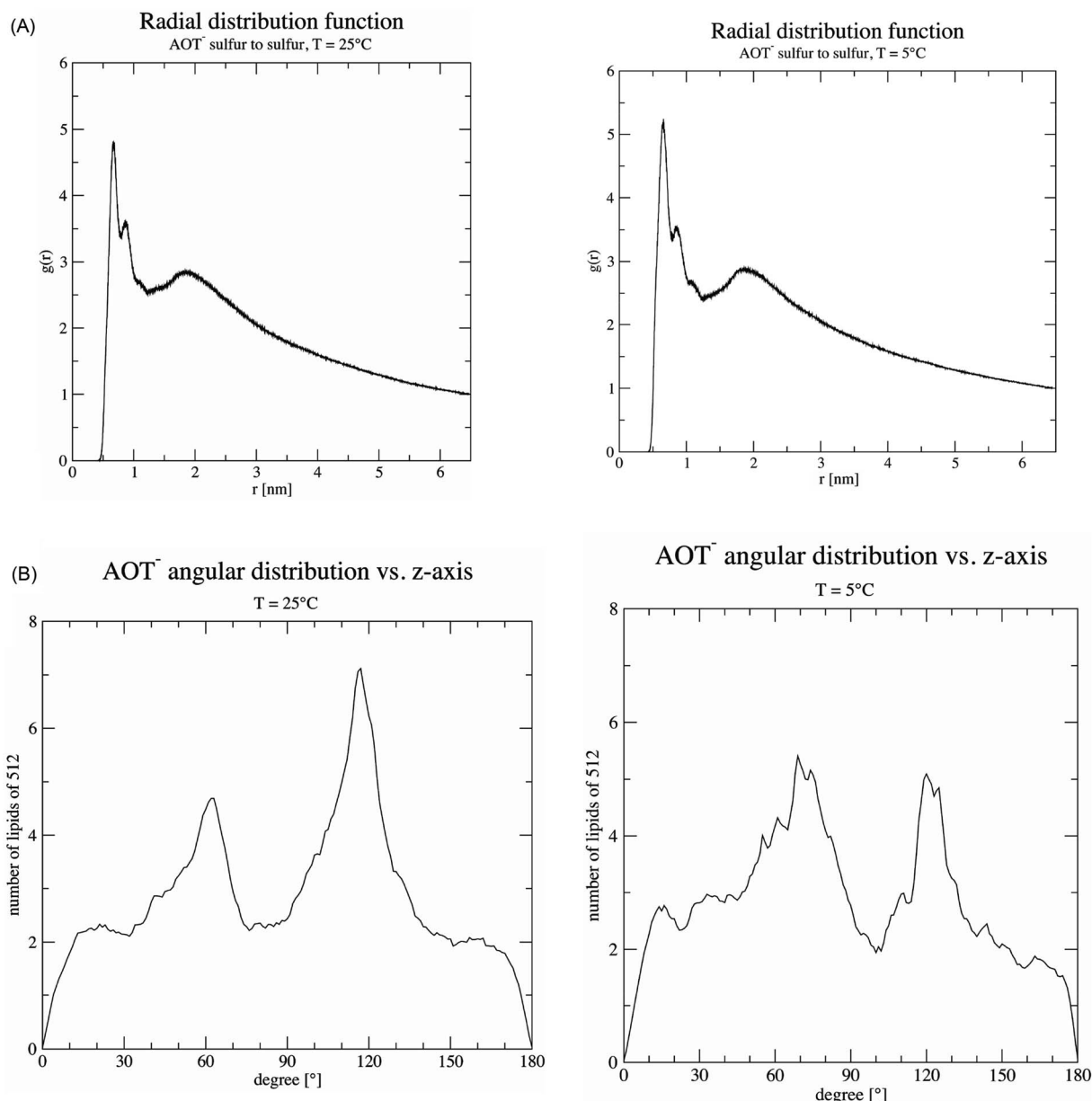
Fig. 9 Effect of temperature. (A) The radial distribution function of sulfur atoms reveals the average distances between the AOT head groups. For AOT membranes at T = 25\text{ }^{\circ}\text{C} , the distances are similar with a value of 0.664 nm compared to 0.662 nm at T = 5\text{ }^{\circ}\text{C} . The peak at T = 5\text{ }^{\circ}\text{C} ( g(r) > 5 ) is higher than at T = 25\text{ }^{\circ}\text{C} ( g(r) < 5 ), indicating that at T = 5\text{ }^{\circ}\text{C} more than 5 AOT molecules surround each AOT at the similar distance (average g(r) = 5.20 ). At T = 25\text{ }^{\circ}\text{C} temperature, the peak height is "softer"; and there are below 5 surrounding AOT in the vicinity of each AOT (average g(r) = 4.81 ). (B) The preferred orientation of AOT compared to the z-axis, for both temperatures, is more pronounced at 60 and 120°, than around 90° (flat) against the z-axis. The drop at exactly the z-axis must be ignored, its origin are numerical instabilities of the calculation due to divisions close to zero. At T = 5\text{ }^{\circ}\text{C} , it seems that the angular distribution (peak height) has become a bit more equal than at T = 25\text{ }^{\circ}\text{C} .
