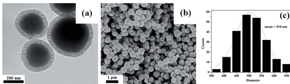
Fig. 1 TEM and SEM of \text{Fe}_3\text{O}_4@m\text{SiO}_2@m\text{SiO}_2\text{-CD} (a and b), and the size distribution histogram of \text{Fe}_3\text{O}_4@m\text{SiO}_2@m\text{SiO}_2\text{-CD} microspheres calculated from SEM images (c).
