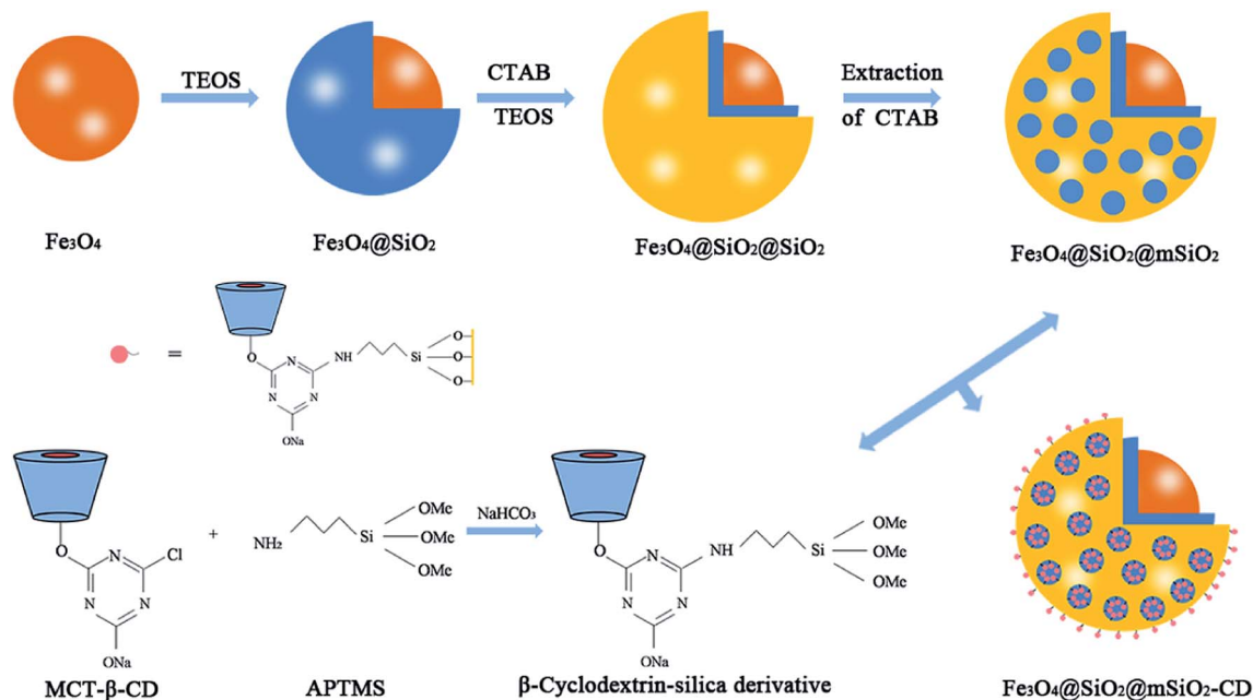
Scheme 1 Schematic illustration of the formation of \text{Fe}_3\text{O}_4@m\text{SiO}_2@m\text{SiO}_2\text{-CD} microspheres.
