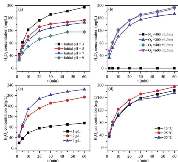
Fig. 7 Effect of (a) pH, (b) oxygen flow rate, (c) Mg-CNT composite dosage and (d) operational temperature on the accumulation of in situ generated \text{H}_2\text{O}_2 .
