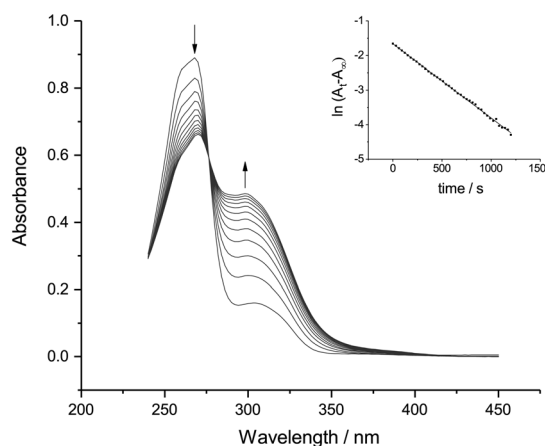
Fig. 4 UV-Vis spectra of p -CBD tetrafluoroborate ( 70 \mu\text{M} ) in 50% (v/v) ACN-aqueous phosphate buffer ( 0.05 \text{ M} , \text{pH}_{\text{obs}} 7.8). Scans were repeated every two minutes at 22.5 \pm 0.5^\circ \text{C} . Inset: first-order rate plot of the disappearance of the p -CBD peak at 268 \text{ nm} .
