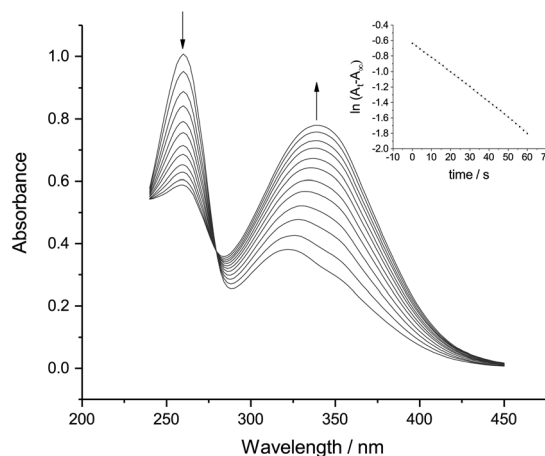
Fig. 3 UV-Vis spectra of p -NBD tetrafluoroborate ( 70 \mu\text{M} ) in 50% (v/v) ACN-aqueous phosphate buffer ( 0.05 \text{ M} , \text{pH}_{\text{obs}} 7.8). Scans were repeated every five seconds at 22.5 \pm 0.5^\circ \text{C} . Inset: first-order rate plot of the disappearance of the p -NBD peak at 260 \text{ nm} .
