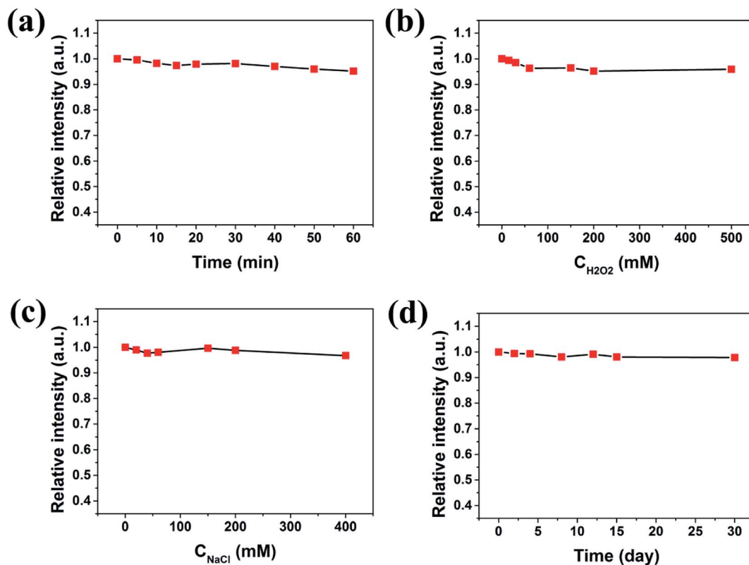
Fig. 2 (a) Effect of time intervals of irradiation with a UV lamp on fluorescence intensity of PNCs. (b) Effect of oxidant on the fluorescence intensity of PNCs. (c) Effect of ionic strengths on the fluorescence intensity of PNCs (ionic strengths were controlled by various concentrations of NaCl in aqueous solution). (d) Effects of storage time on the fluorescence intensity of the PNCs.
