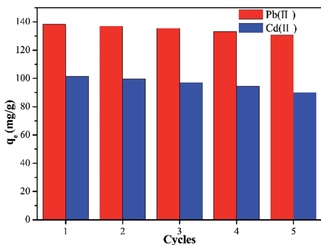
Fig. 8 Adsorption capacity of Pb(II) and Cd(II) onto Y- \beta -CDP with five adsorption-desorption cycles.
