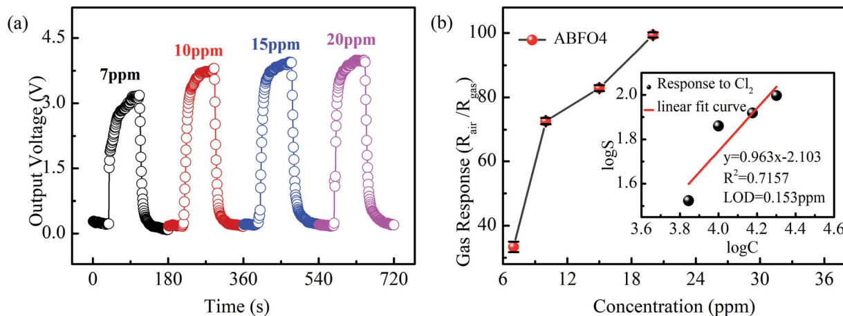
Fig. 5 (a) Typical response and recovery curve of sensors and (b) sensitivity pattern of ABFO4 to \text{Cl}_2 as the concentration varied from 7 ppm to 20 ppm at 240^\circ\text{C} .
