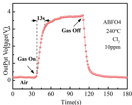
Fig. 6 The response time of ABFO4 exposed to 10 ppm \text{Cl}_2 at 240^\circ\text{C} .
