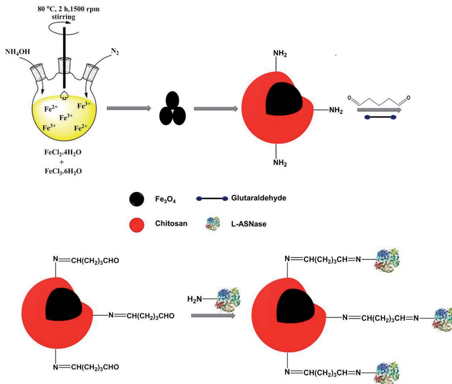
Fig. 1 Immobilization of L-ASNase onto the magnetic Fe 3 O 4 -chitosan core-shell particles.
