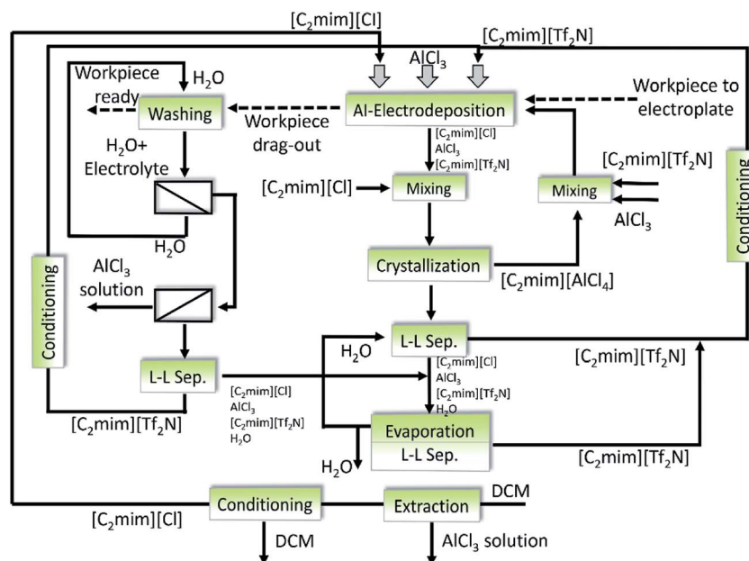
Fig. 22 Complete recycling concept for the [\text{C}_2\text{mim}][\text{Tf}_2\text{N}] - \text{AlCl}_3 -based electrolytes in aluminum electrodeposition. Reproduced with permission from ref. 208. Copyright 2010 WILEY-VCH.
