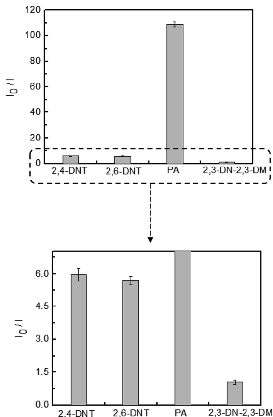
Fig. 5 Relative changes in fluorescence intensity of TPE-CMP ( 0.375 \text{ mg mL}^{-1} in \text{CH}_2\text{Cl}_2 ) upon exposure to 2,4-DNT, 2,6-DNT, PA, and 2,3-DN-2,3-DM. [Explosives] = 2.5 \times 10^{-3} \text{ M} . Excitation wavelength 330 nm. I_0 and I represent fluorescence intensity at 550 nm before and after exposure to explosives, respectively.
